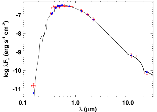
Figure 5. Spectral energy distribution of \lambda Ser. Red symbols represent the observed photometric measurements, where the horizontal bars represent the effective width of the passband. Blue symbols are the model fluxes from the best-fit Kurucz atmosphere model (black).
