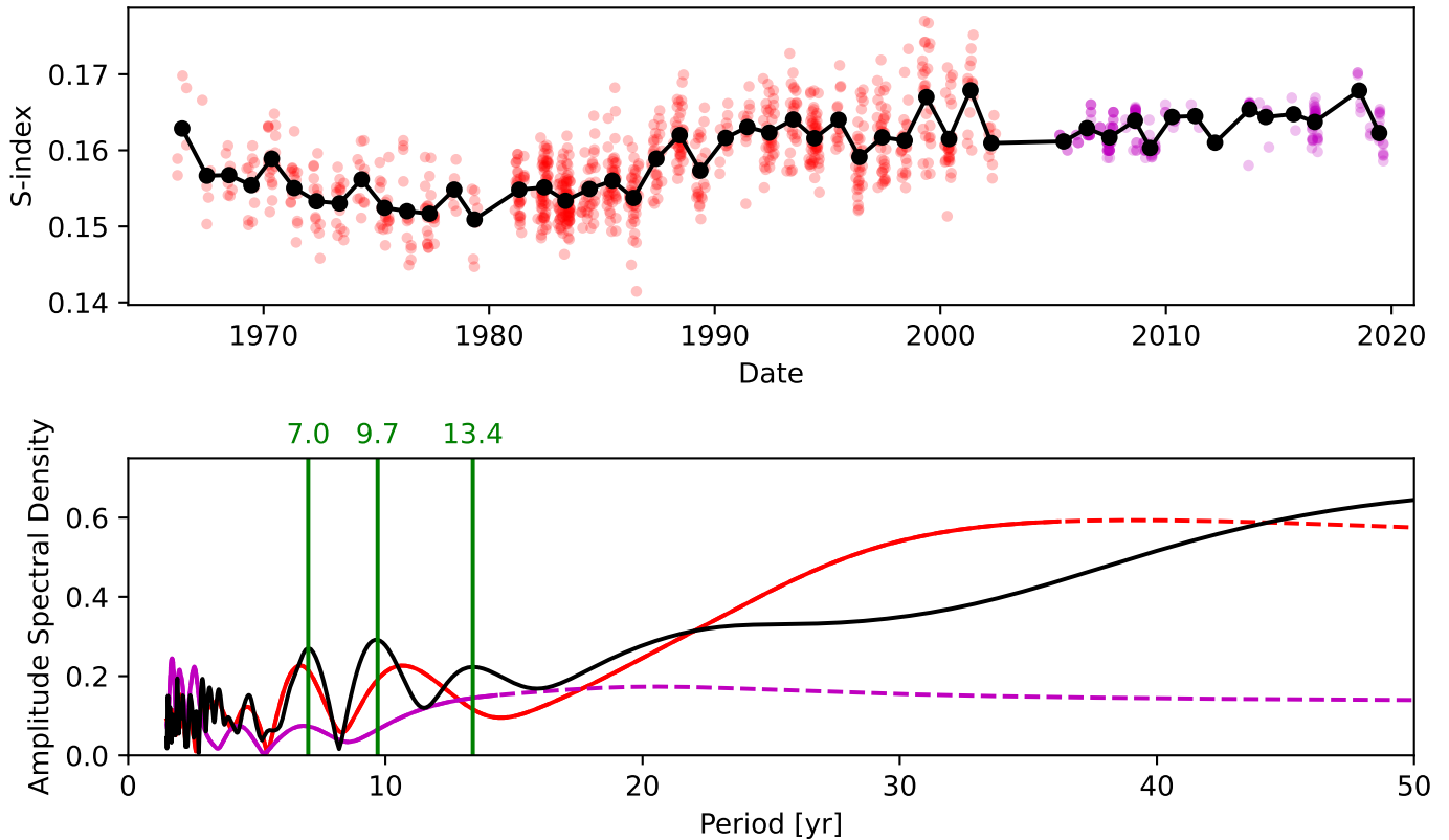
Figure 4. Top: 54-year S -index time series for \lambda Ser. Observations are shown from MWO HKP (red) and Keck HIRES-2 (purple) with seasonal means (black). Bottom: Lomb-Scargle periodogram of the time series, with MWO-only in red, Keck-only in purple, and the composite time series in black. Dashed lines indicate portions of the periodogram beyond the duration of the time series. The top three peaks in the composite time series are indicated with green vertical lines. The periodogram is expressed in units of signal amplitude normalized by a standard deviation.
