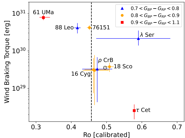
Figure 8. Evolution of the wind braking torque with Ro from the calibration of Corsaro et al. (2021). Points are grouped by Gaia color, corresponding to solar analogs (yellow circles), and hotter (blue triangles) or cooler stars (red squares). The empirical constraint for Ro_{\text{crit}} on this scale is shown with a vertical dashed line.
