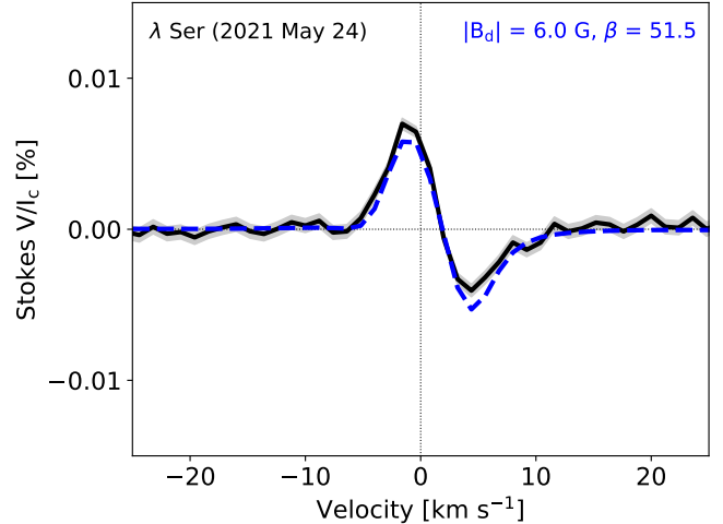
Figure 2. Stokes V polarization profile for \lambda Ser from LBT observations on 2021 May 24. The mean profile is shown as a black line, with uncertainties indicated by the gray shaded area. The blue line is a model profile assuming dipole geometry and fixed inclination.
