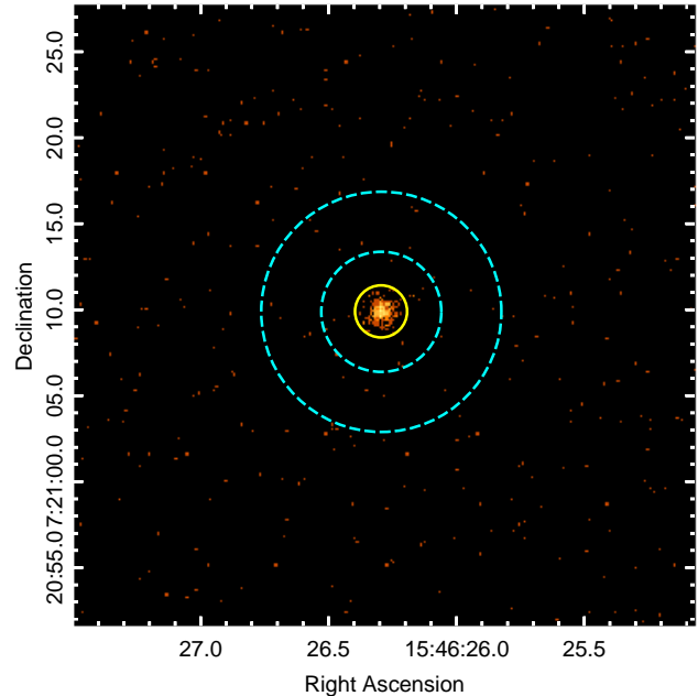
Figure 3. Chandra HRC-I image of \lambda Ser illustrating the source and innermost of two background regions used for the count rate measurement (see Section 2.3 for details).
