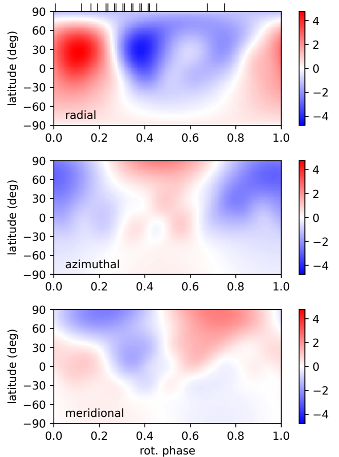
Figure 7. Large-scale surface magnetic geometry of \lambda Ser. The three panels display the field components in spherical coordinates, adopting an equatorial projection. Color bars on the right show the field strength in Gauss. Vertical ticks above the top panel indicate observed rotational phases.
