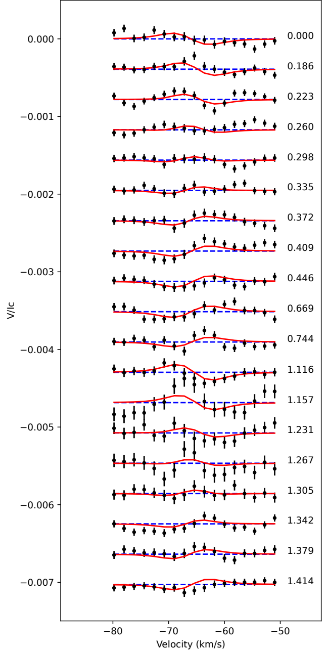
Figure 6. Stokes V LSD profiles obtained with Neo-NARVAL (black dots), and synthetic profiles produced by ZDI (red curves). Successive observations are vertically shifted for clarity, and the rotational phase \Phi of the observation is listed along the right side.
