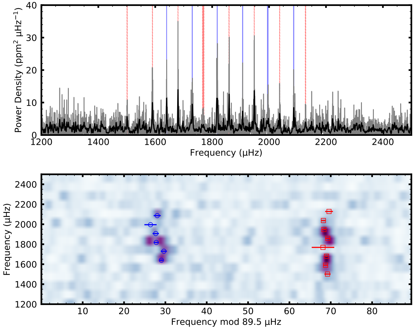
Figure 1. Power spectrum (top) and échelle diagram (bottom) centered on the power excess due to solar-like oscillations detected in \lambda Ser. Blue solid lines and circles indicate extracted radial ( l = 0 ) modes, while red dashed lines and squares show extracted dipole ( l = 1 ) modes.
