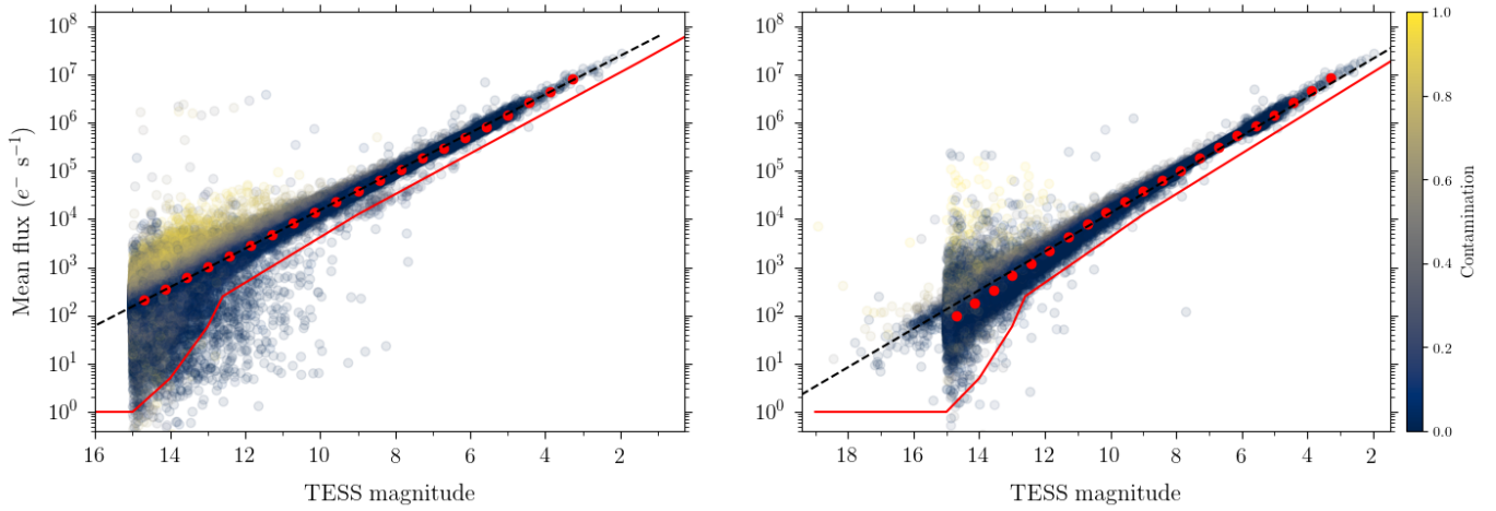
Figure 12. Relation between extracted flux from simple aperture photometry and the TESS magnitude, color-coded by contamination, here for Sector 3 data. The left (right) panels show values for 1800-sec (120-sec) data. The black dashed line gives the relations obtained following the prescription in Equation (4), which has been fitted to the red median binned points. The full red line gives the adopted boundary for the data validation.
